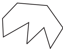
NONAGON
