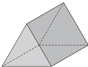
TRIANGULAR PRISM
